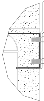
DETAIL A SCALE 0,300 HANGING SOLUTION A
